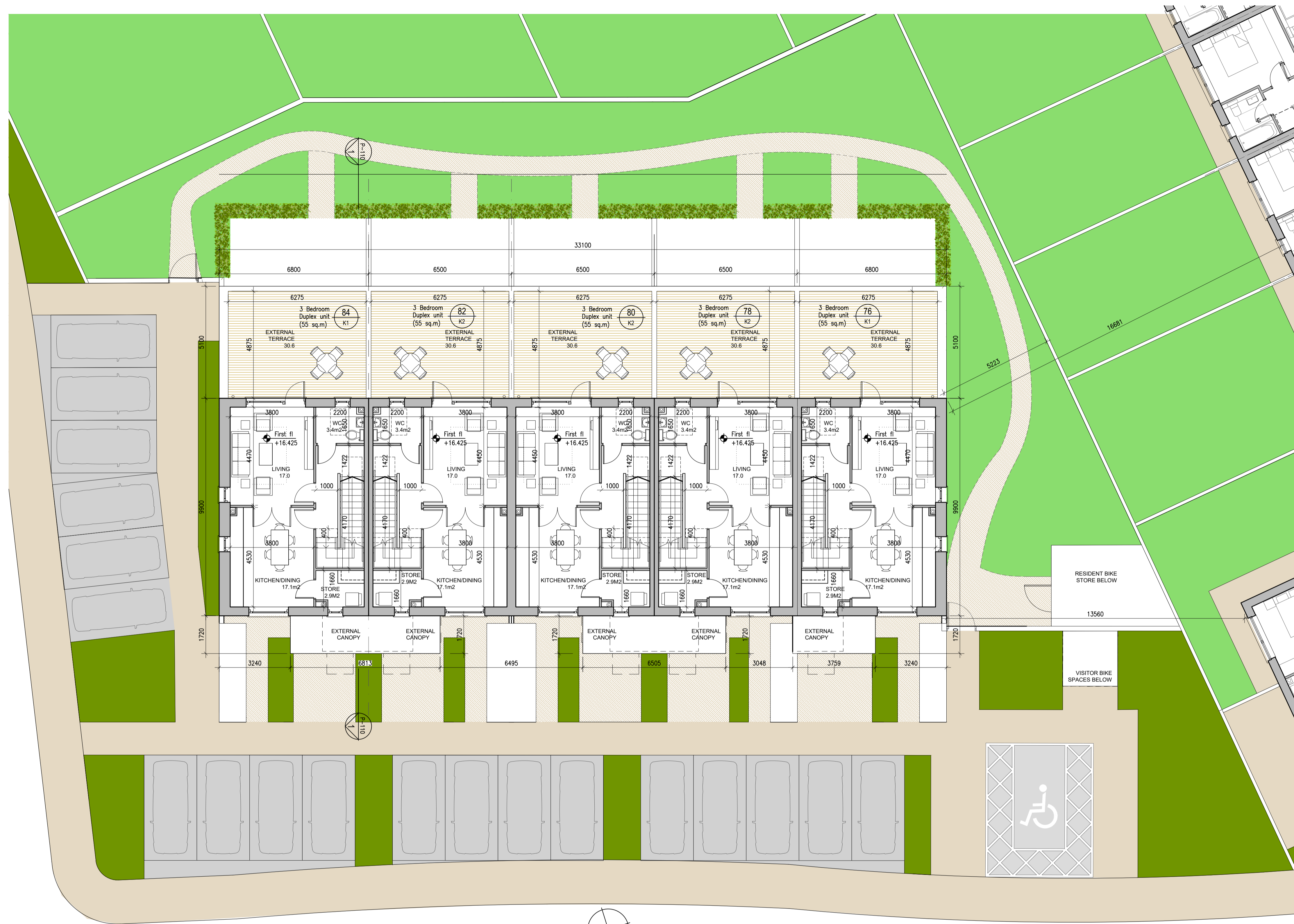
02 107 1:100@A1 2 & 3 BED DUPLEX UNIT
